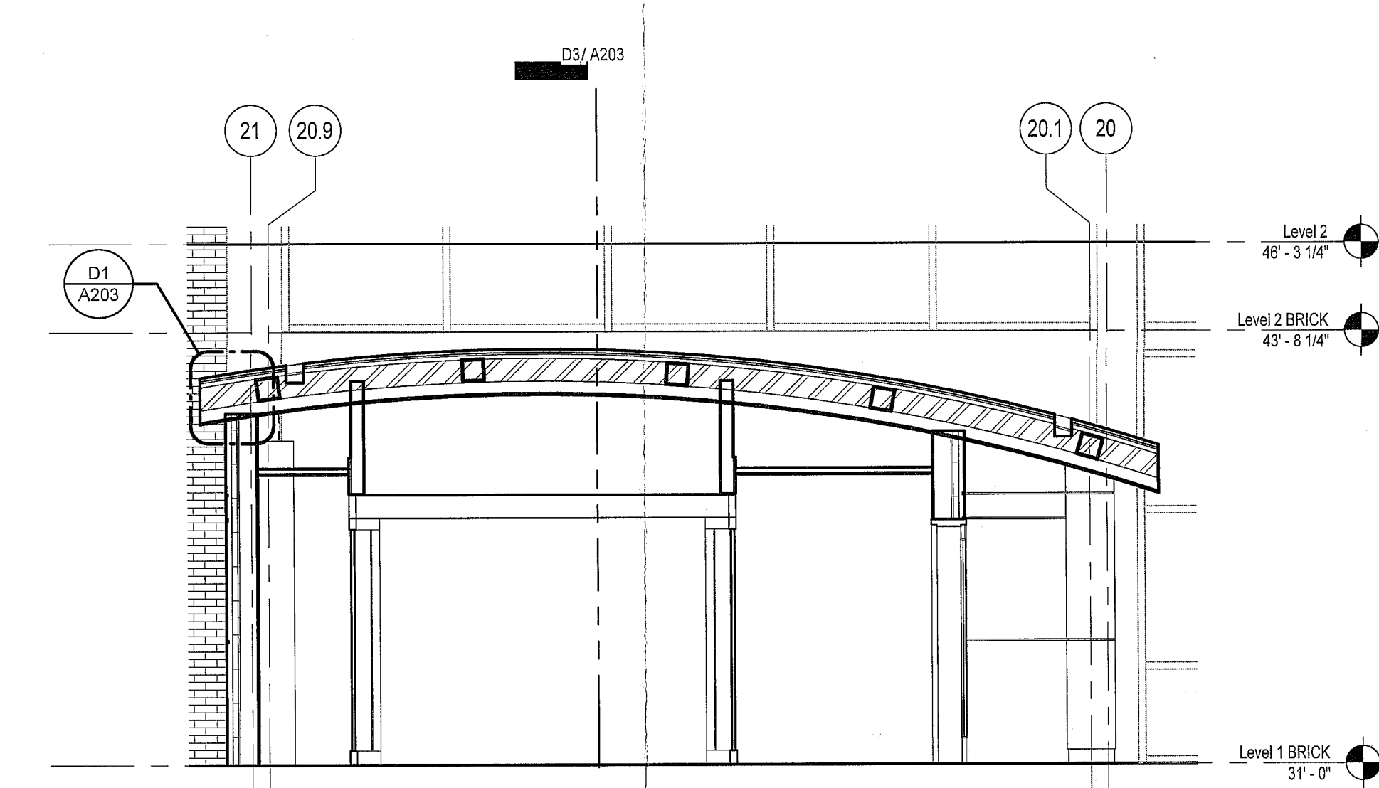
D4 CANOPY SECTION, NORTH/SOUTH SCALE: 1/4" = 1'-0"
