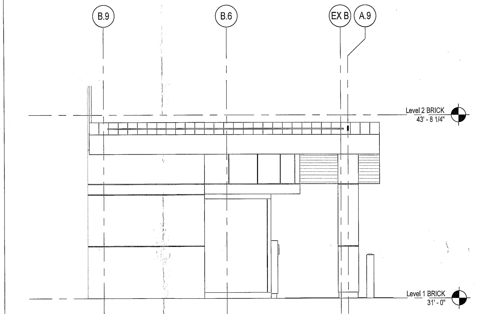
C3 CANOPY NORTH ELEVATION SCALE: 1/4" = 1'-0"
