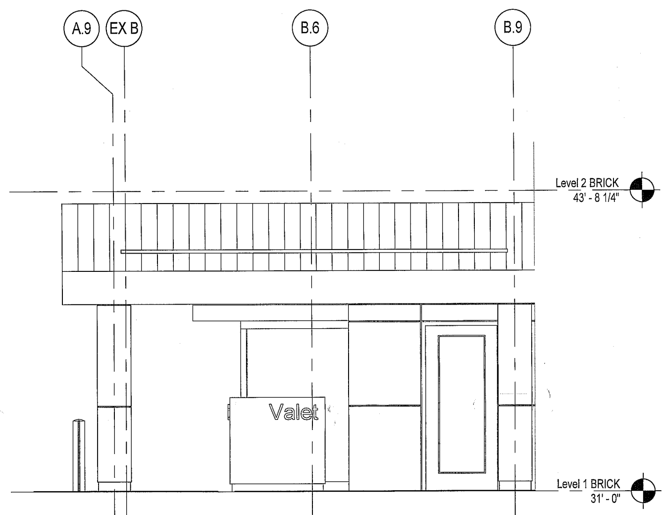
C2 CANOPY SOUTH ELEVATION SCALE: 1/4" = 1'-0"
