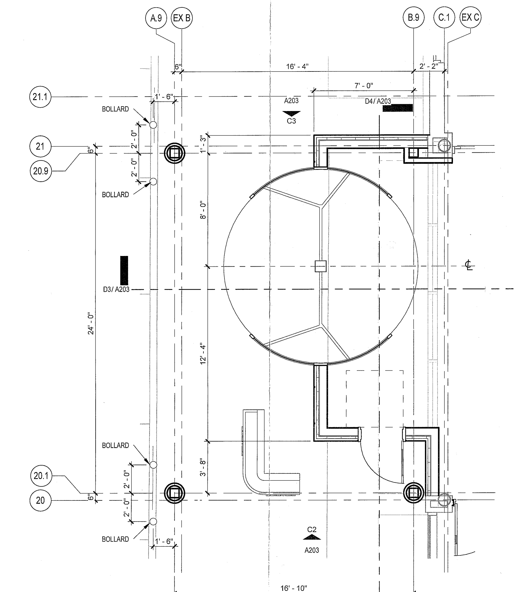
A4 CANOPY FLOOR PLAN SCALE: 1/4" = 1'-0"
