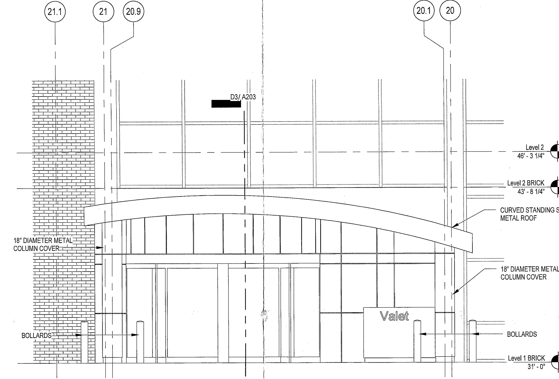
C4 CANOPY WEST ELEVATION SCALE: 1/4" = 1'-0"
