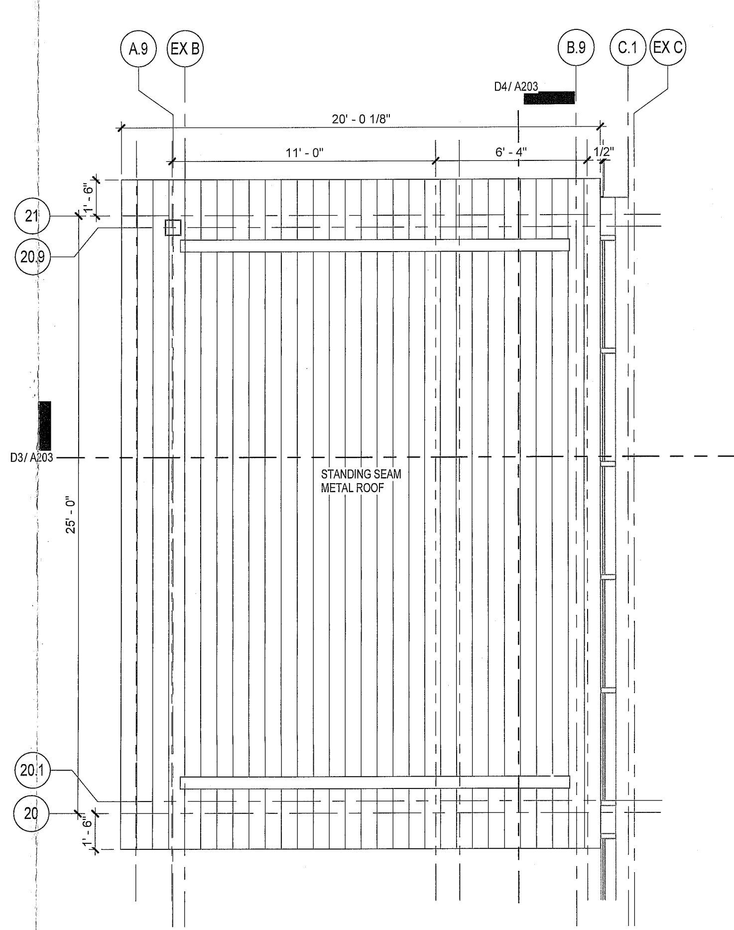
A2 CANOPY ROOF PLAN SCALE: 1/4" = 1'-0"
