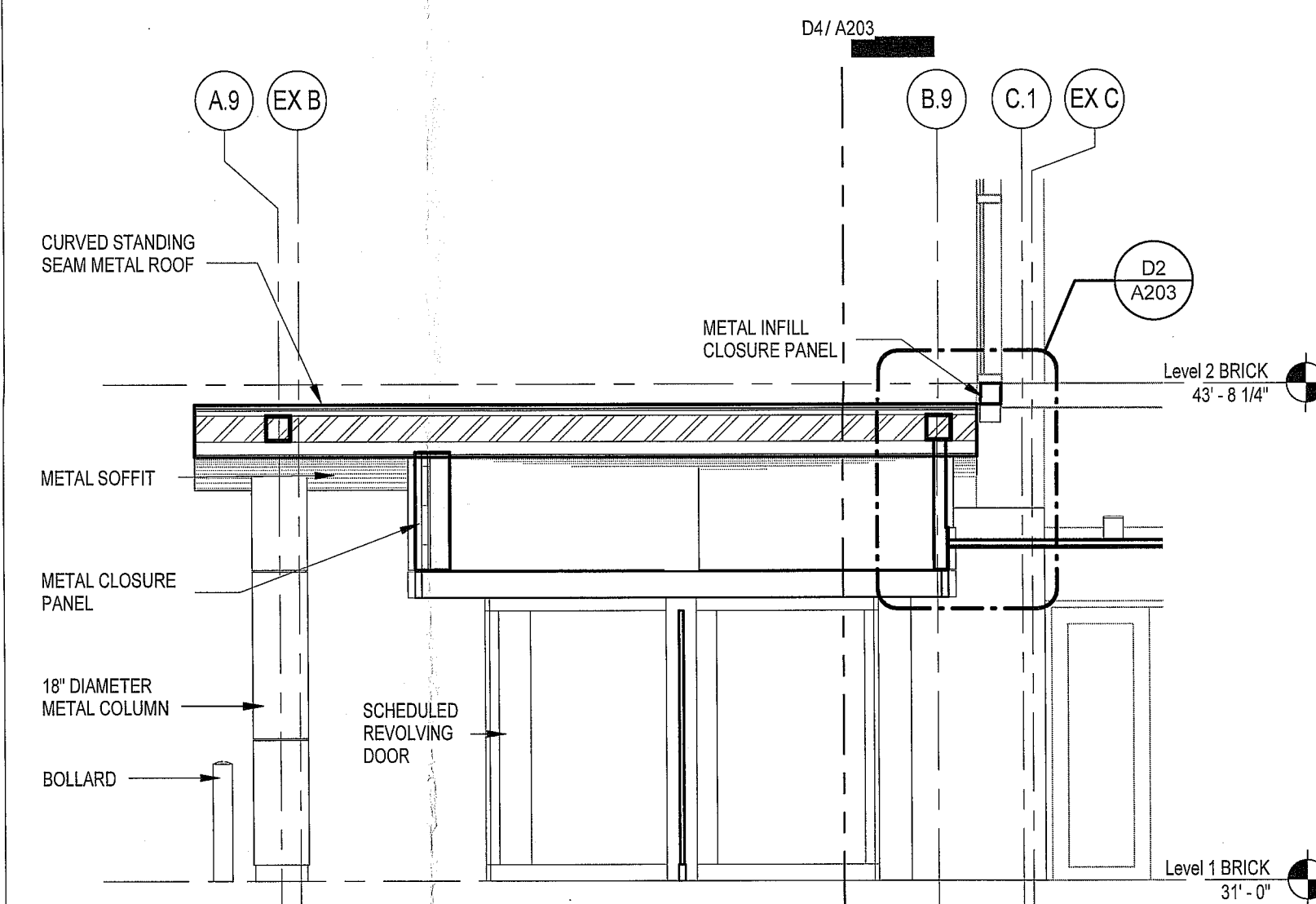
D3 CANOPY SECTION, EAST/WEST SCALE: 1/4" = 1'-0"
