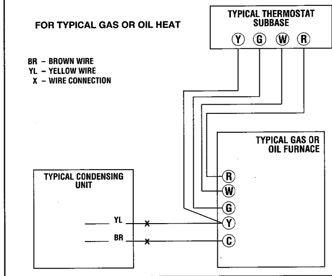
FIGURE 2 CONTROL WIRING FOR GAS OR OIL FURNACE
