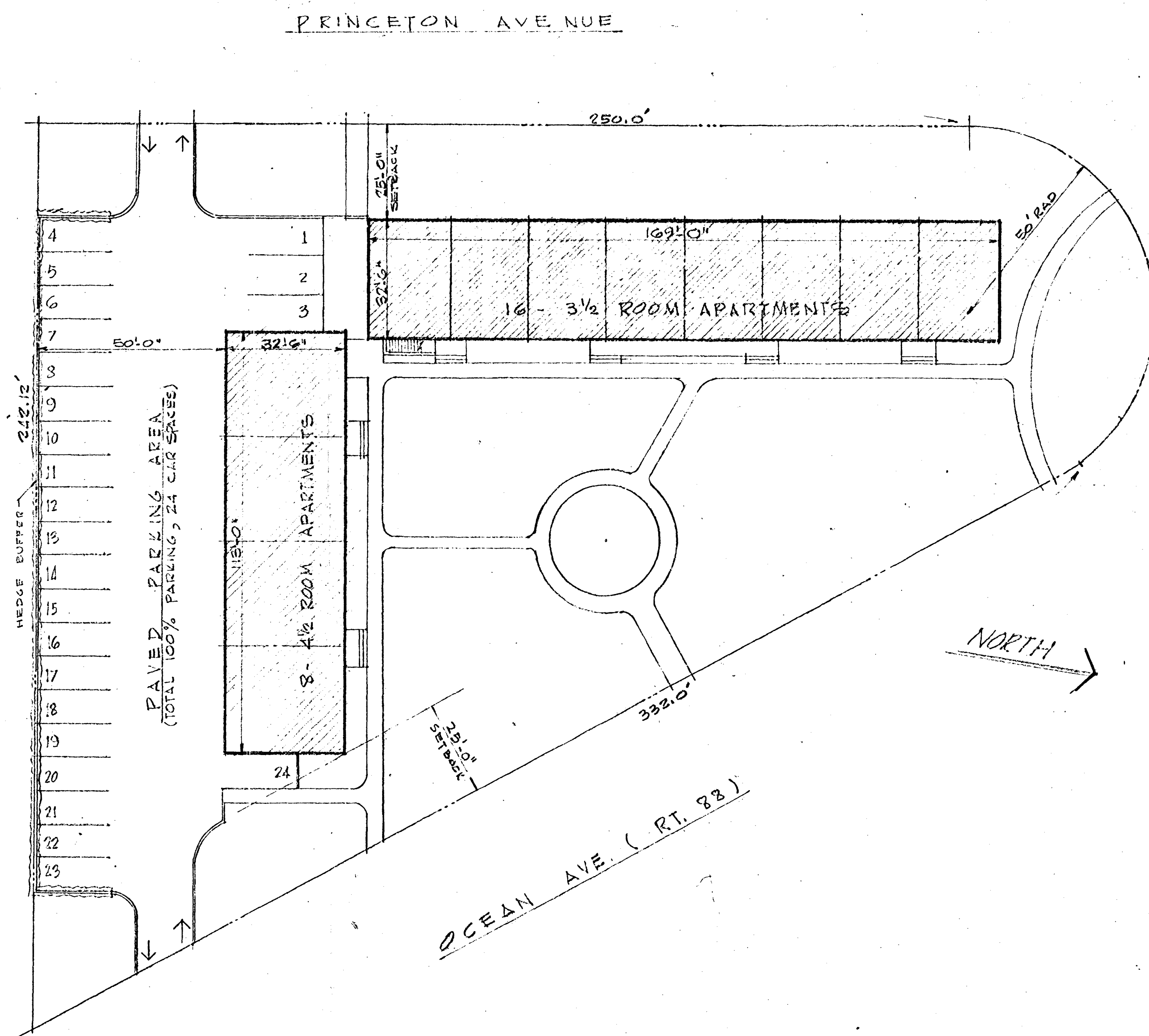
PLOT PLAN SCALE 1" = 20'-0"
