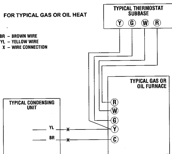
FIGURE 2 CONTROL WIRING FOR GAS OR OIL FURNACE
