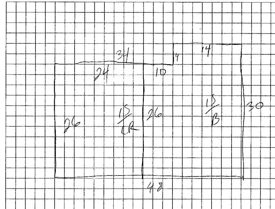
01.00 FLOOR DIMENSIONS
