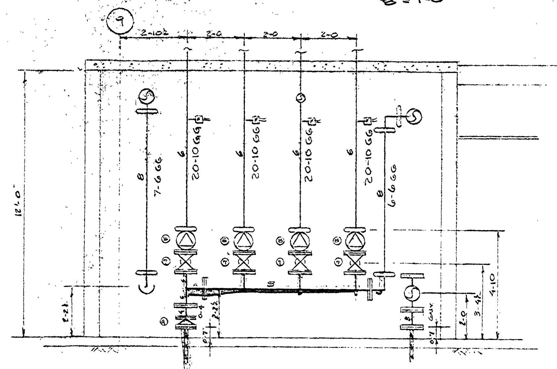
SECTION B-B 1/8" = 1'-0"
