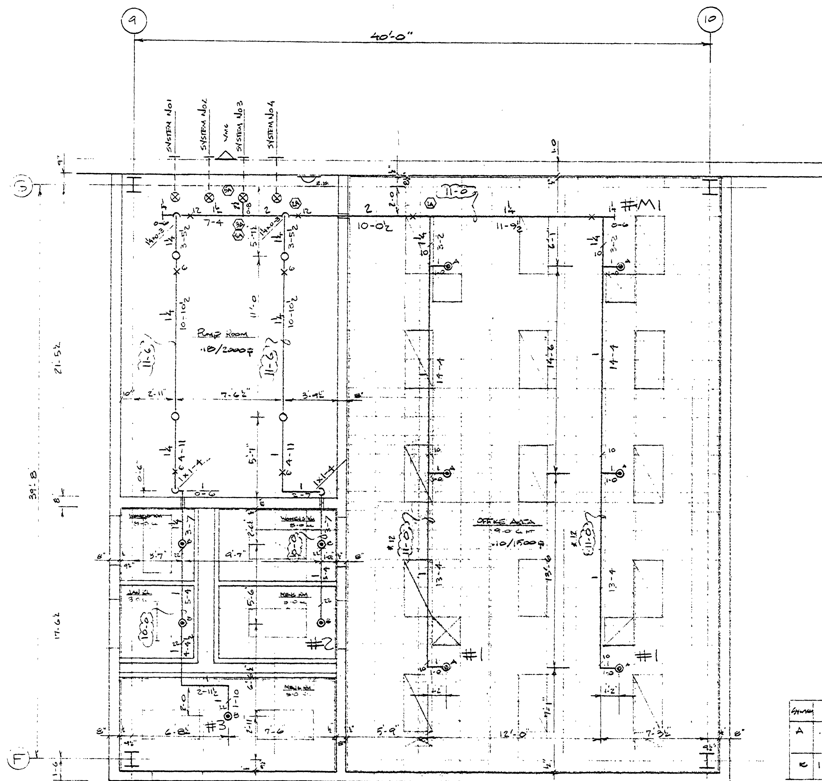
OFFICE AREA 1/4" = 1'-0"
