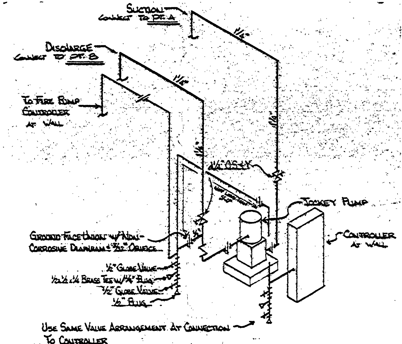
Jockey Pump & Base Rate 1/4" = 1'-0"
