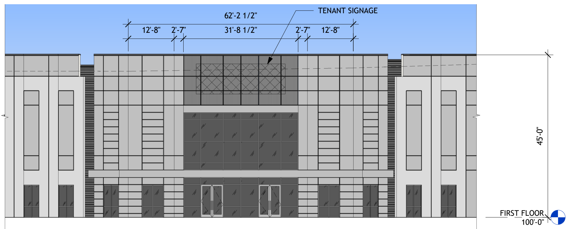
5 CORNER ELEVATION 1/16" = 1'-0"
