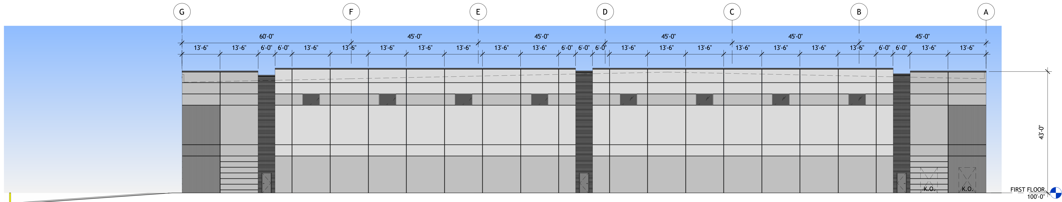
4 SOUTH ELEVATION 1/16" = 1'-0"
