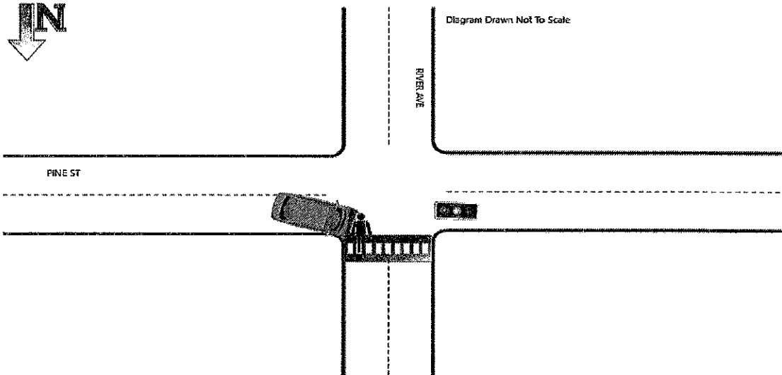
144 Crash Diagram (NOT TO SCALE)
