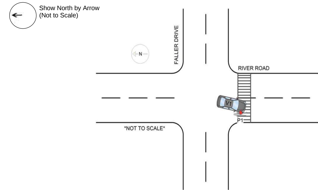
144 Crash Diagram
