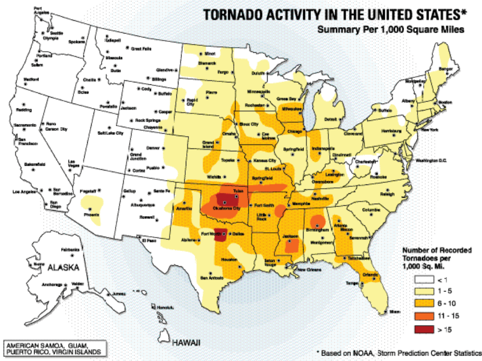
Figure 4.3 - 3 Tornado Activity in the United States
