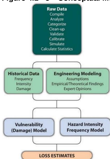
Figure 4.1 - 5 Conceptual Model of the Statistical Risk Assessment Methodology
