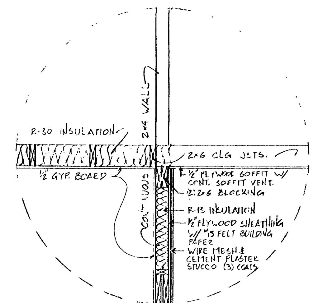
B KNEE WALL & SOFFIT DETAIL SCALE: 3/4"=1'-0"
