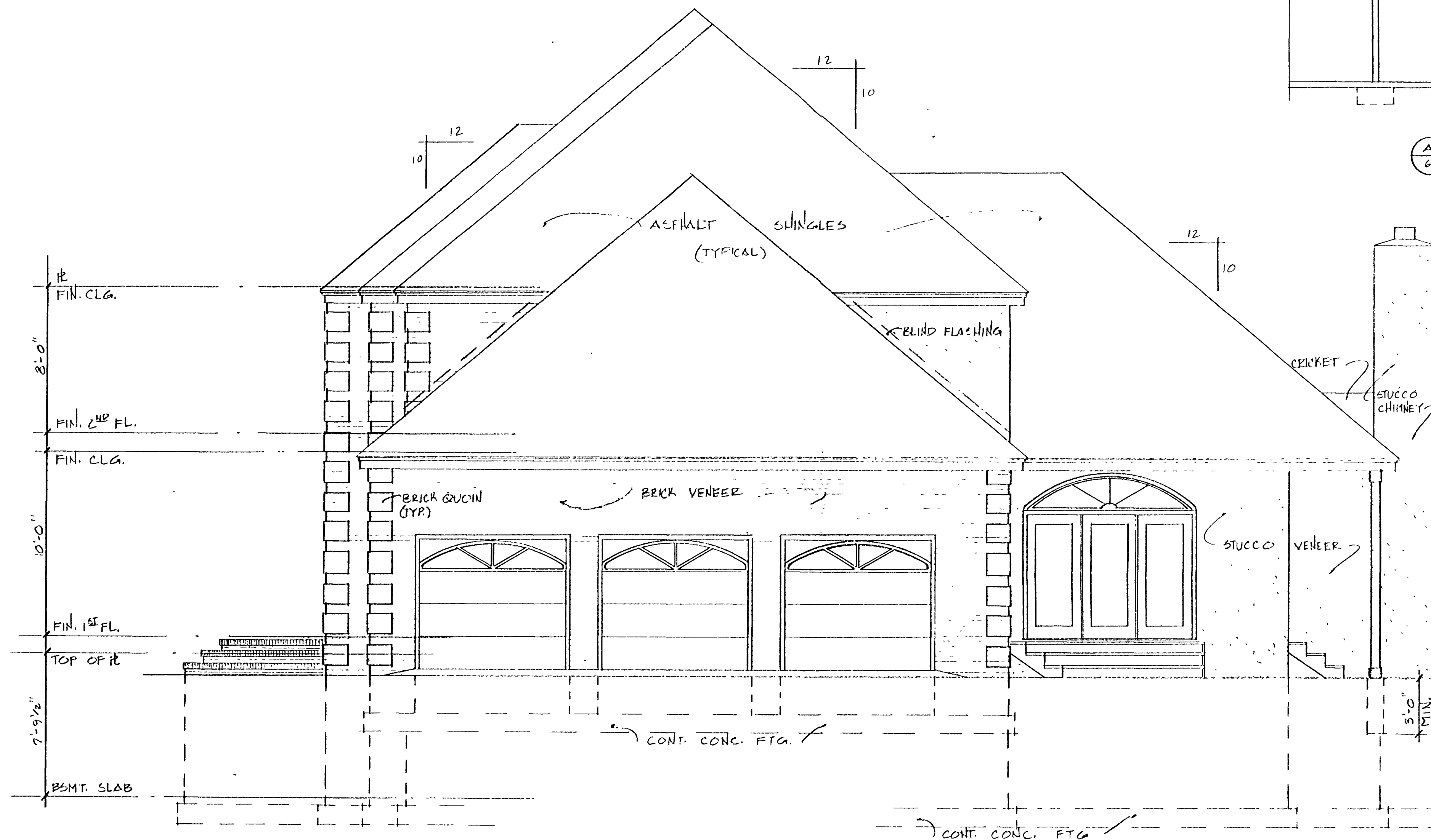
RIGHT SIDE ELEVATION 1/4"=1'-0"
