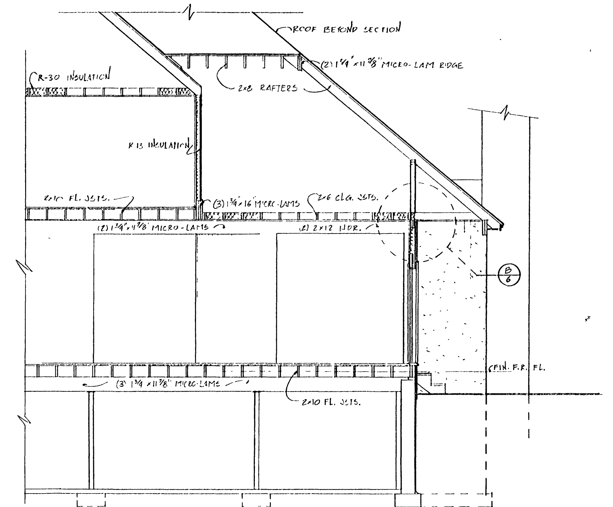
A BUILDING SECTION SCALE: 1/4"=1'-0"
