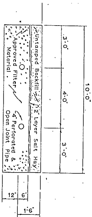
TYPICAL SECTION-DISPOSAL BED
